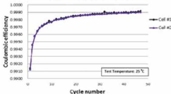
Coulombic Efficiency Measurement
